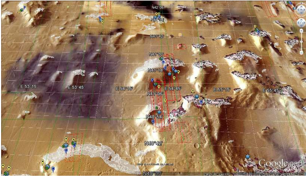
Figure 3.9: An area of Protonilus Mensae, showing areas where segments are selected for having a northerly aspect and a relatively steep slope of more than 10 degrees. In this figure the head and termini locations are marked with blue and yellow markers respectively, and the centre with a snowflake.
