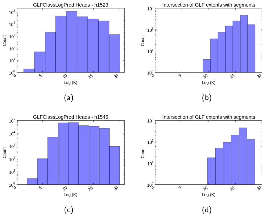
Figure 4.22: Histogram of \log_e(K_h) for tiles h1523 and h1545 calculated based on the 100m buffer around the heads.
