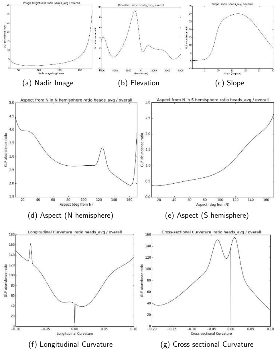
Figure 4.4: Ratio of Souness GLF counts to overall HRSC histograms as functions of feature vector variables - 100m radius head buffers.
