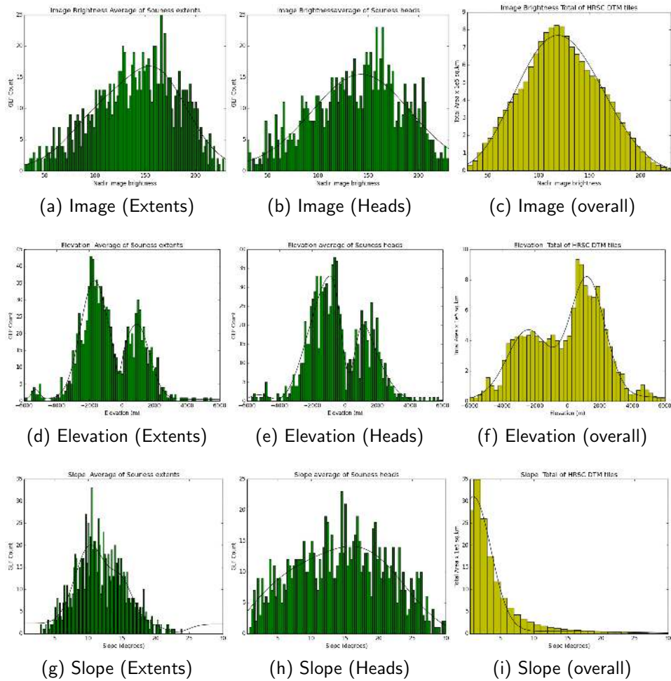
Figure 4.1: Histograms showing average brightness of nadir image, elevation, and slope over Souness GLF extents, over 100m radius buffers around Souness head locations, and over all pixels summed by area in the HRSC DTM tiles.
