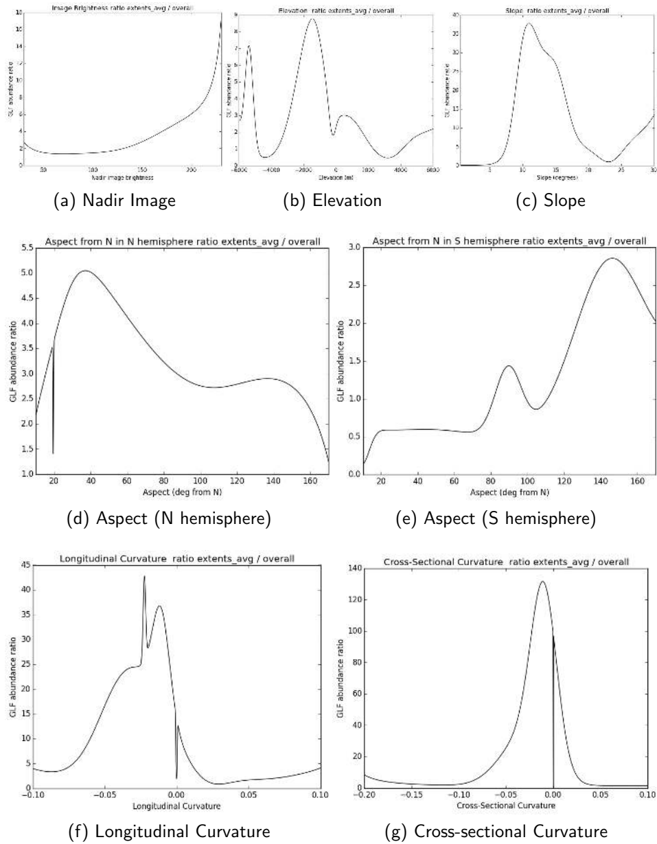
Figure 4.3: Ratio of Souness GLF counts to overall HRSC histograms as functions of feature vector variables - extents.
