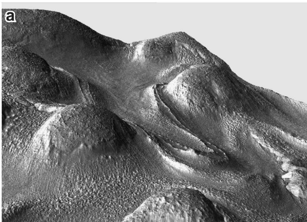
Figure 2.4: A figure from Hubbard et al. (2011) showing the location of a GLF complex on the north wall of the southern hemisphere crater Greg, and a 3D perspective rendering of one of the GLFs.
