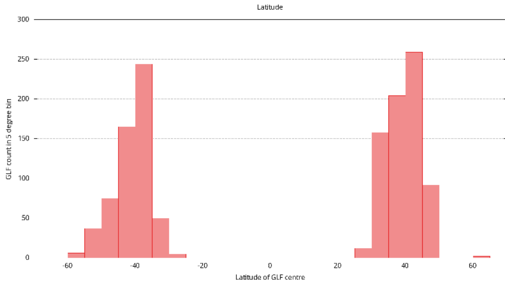
Figure 5.2: The distribution of the Souness GLF centre latitudes, including all 1309 objects. The southern hemisphere distribution continues to lower latitudes, however the flat, low topography in the northern hemisphere may be responsible for this rather than being a primary effect of latitude.
