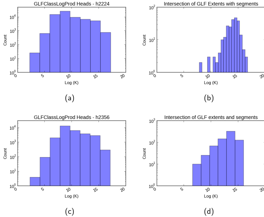
Figure 4.19: Histograms of \log_e(K_h) for tiles h2224 and h2356 calculated based on the 100m buffer around the heads.
