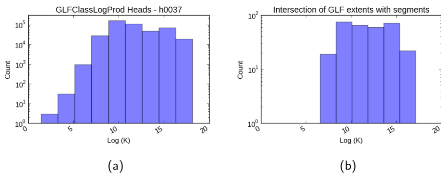
Figure 4.16: Histogram of \log_e(K_h) for tile h0037 calculated based on the 100m buffer around the heads. The mean and standard deviation of \log_e(K_h) are 10.65 and 5.44 respectively. The number of segments intersecting is 608 and the mean and standard deviation of \log_e(K_h) for these are 11.53 and 3.55.
