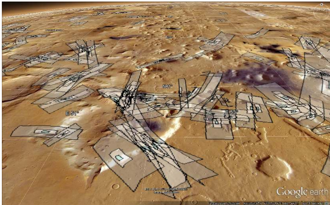
Figure 3.3: A Google Earth screen shot, showing the Souness GLFs, 'context' and 'context9' shapefile extents in the Protonilus Mensae region of Mars.
