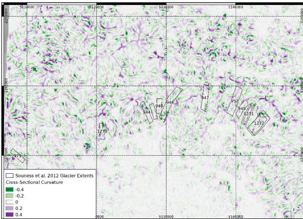
(b) Cross-sectional Curvature
