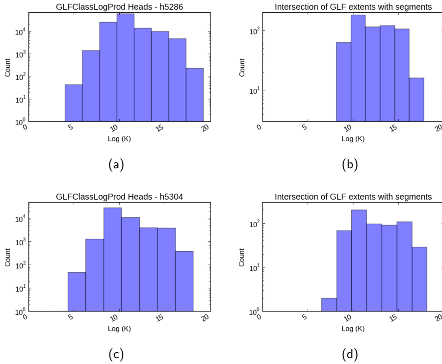
Figure 4.14: Histograms of \log_e(K_h) for tiles h5286 and h5304 calculated based on the 100m buffer around the heads.
