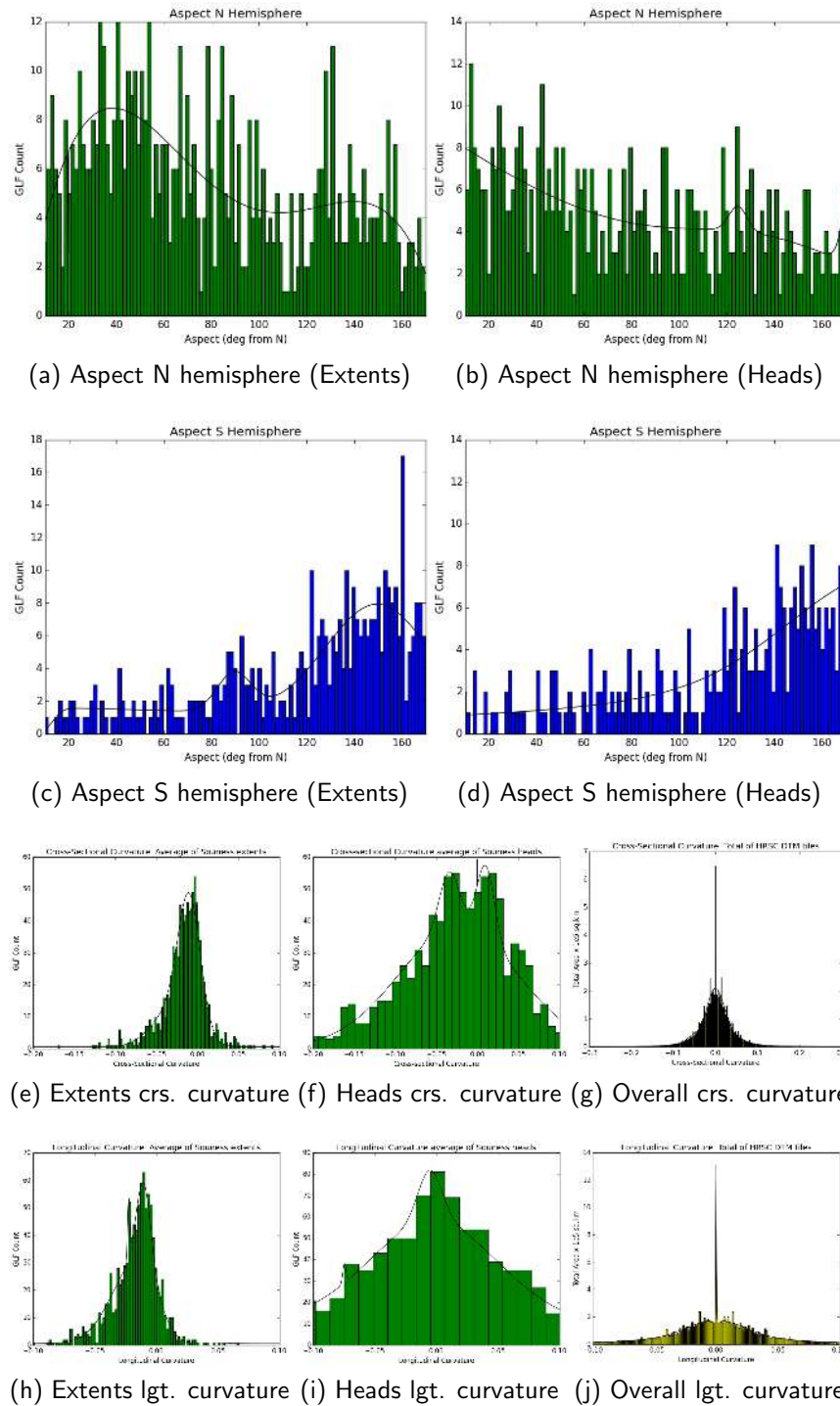
Figure 4.2: Histograms showing average aspect angle from N over Souness GLF extents and heads, in both northern and southern hemispheres, and of the curvature layers for Souness GLF extents and heads and for the HRSC tiles overall. Note that the Souness GLFs have a bias towards negative curvature, whereas the overall data has a symmetric distribution about zero.
