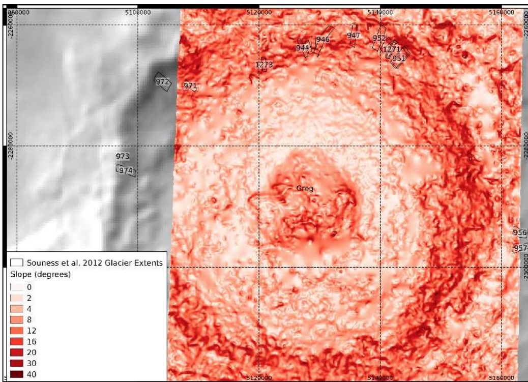
(b) Slope
