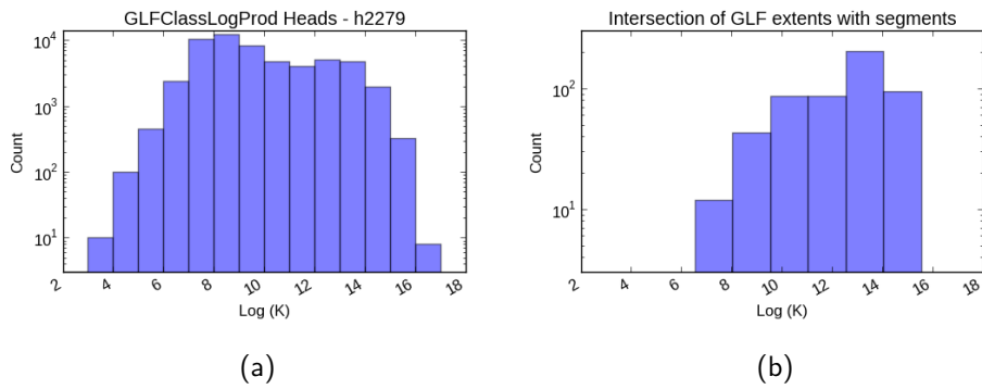
Figure 4.12: Histogram of \log_e(K_h) for tile h2279 calculated based on the 100m buffer around the heads. The mean and standard deviation of \log_e(K_h) are 9.37 and 3.78 respectively. The number of segments intersecting is 531 and the mean and standard deviation of \log_e(K_h) for these are 12.08 and 2.94. The null hypothesis of the intersected segments being the same distribution as the overall tile is rejected at Z = 16.5 .
