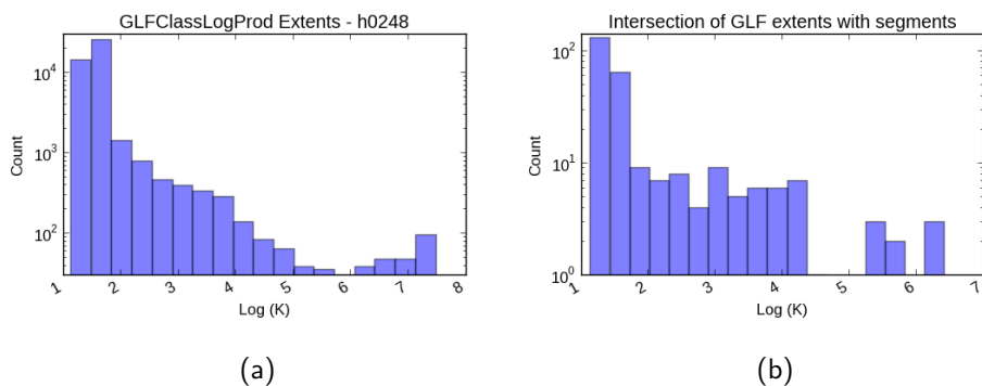
Figure 4.8: Histogram of \log_e(K_e) for tile h0248 calculated based on GLF extents. The mean and standard deviation of \log_e(K_e) are 1.65 and 0.61 respectively. The number of segments intersecting is 263 and the mean and standard deviation of these are 1.86 and 1.08. The Z statistic has a value of 5.58.
