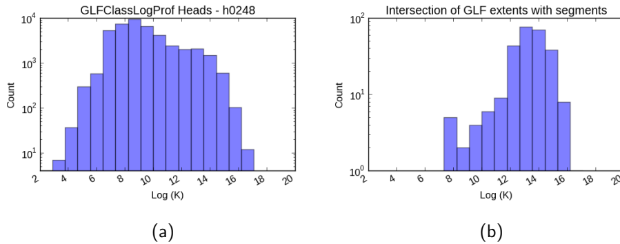
Figure 4.9: Histogram of \log_e(K_h) for h0248 calculated based on the 100m buffer around the heads. The mean and standard deviation are 8.62 and 4.52 respectively. The number of segments intersecting is 263 and the mean and standard deviation of these are 13.24 and 1.46. The Z statistic has a value of 16.6.
